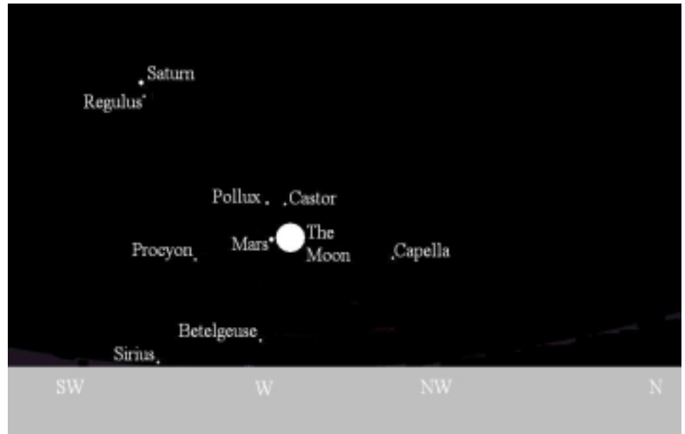
Looking high towards the west about 2½ hours after sunset on April 11, 2008
